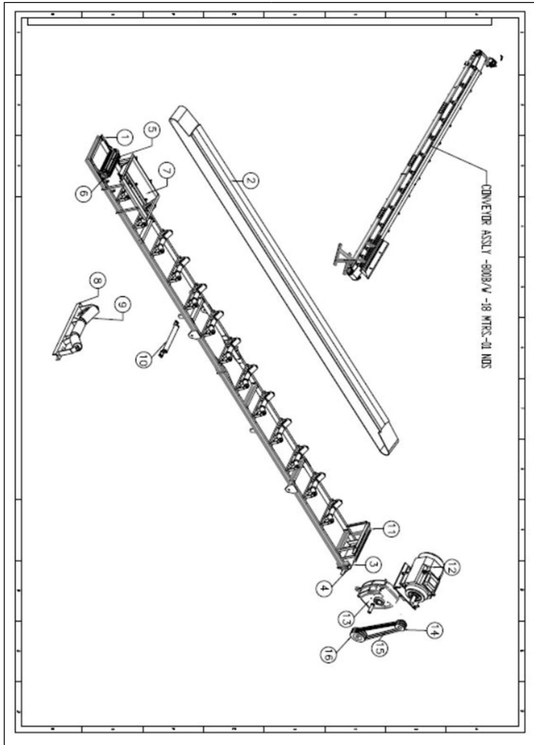
9-CONVEYOR ASSLY (18MX800 B/W) –AJC -BC-A09-01 NO.
